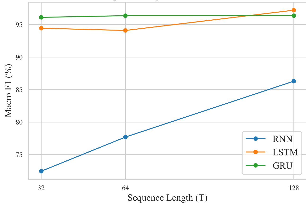
Sequence Length vs. Test F1-score
